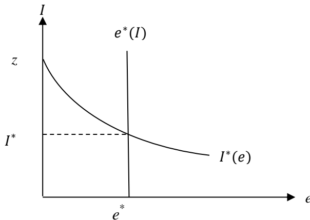
Fig. 1. Reaction functions
